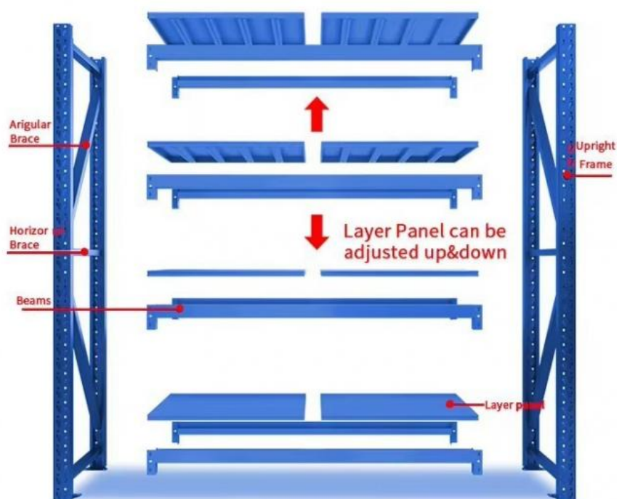
Uprights
